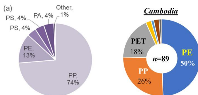
Figure 4. The polymer type distribution analyzed in samples from Mekong River (a), Haberstroh et al. (2021) and in samples from dumping site soils in Cambodia (n = 89) (Cambodia, Tun et al. (2022)). PET: Polyethylene terephthalate, PP: polypropylene, PE: polyethylene, PS: polystyrene, PA: polyamide/nylon and others.
